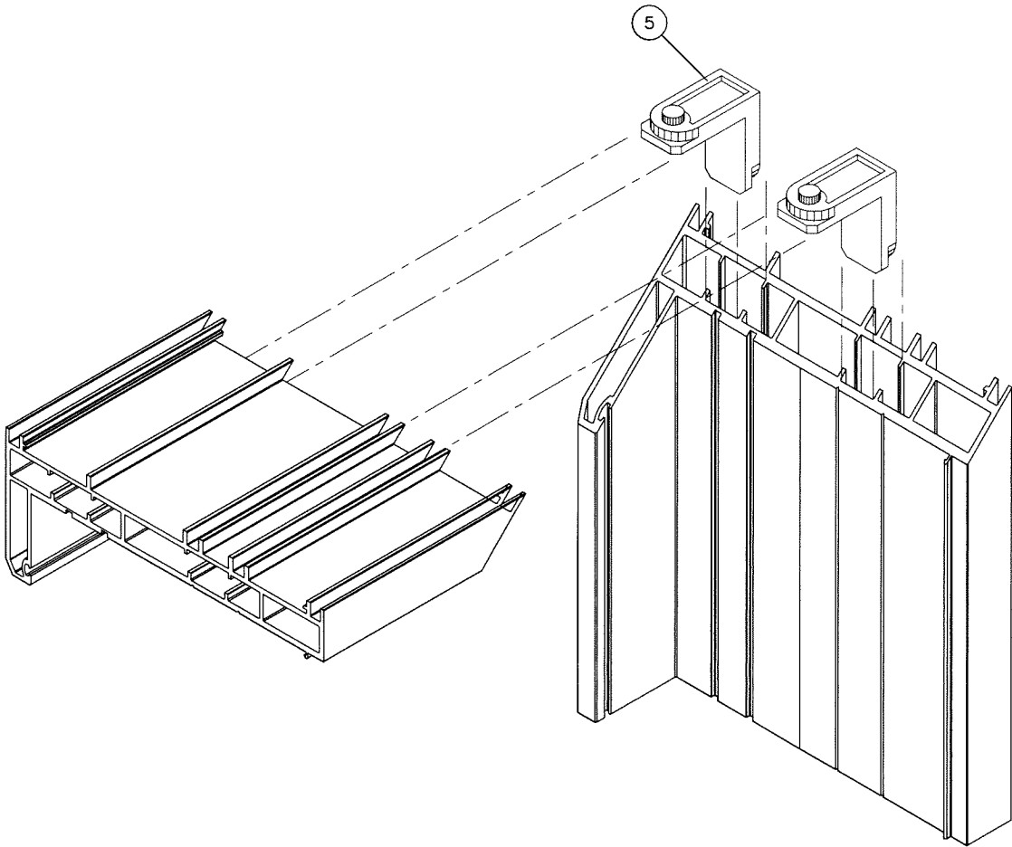
FRAME CORNER
